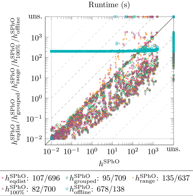
Figure 5: Runtime comparison between the eager SPhO heuristic h^{\text{SPhO}} and our lazy and offline variants on a logarithmic scale. The legend additionally shows the number of tasks a variant solves slower/faster than h^{\text{SPhO}} . Problems that are not solved within the resource limits appear on “uns.” axes.
