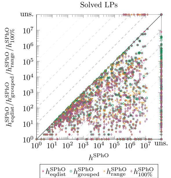
Figure 3: A comparison of the number of solved LPs between the eager SPhO heuristic h^{\text{SPhO}} and all presented lazy versions on a logarithmic scale. Tasks that are not solved within the resource limits appear on “uns.” axes.
