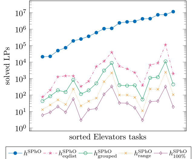
Figure 1: Number of solved LPs in the Elevators domain from the optimal track of IPC 2008 on a log scale. h^{\text{SPhO}} solves an LP for each state, while the four new variants avoid redundant computations.
