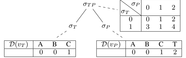
Figure 1: FM \sigma_{TP} over variable space \{T, P\} .
